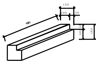
縁石A
